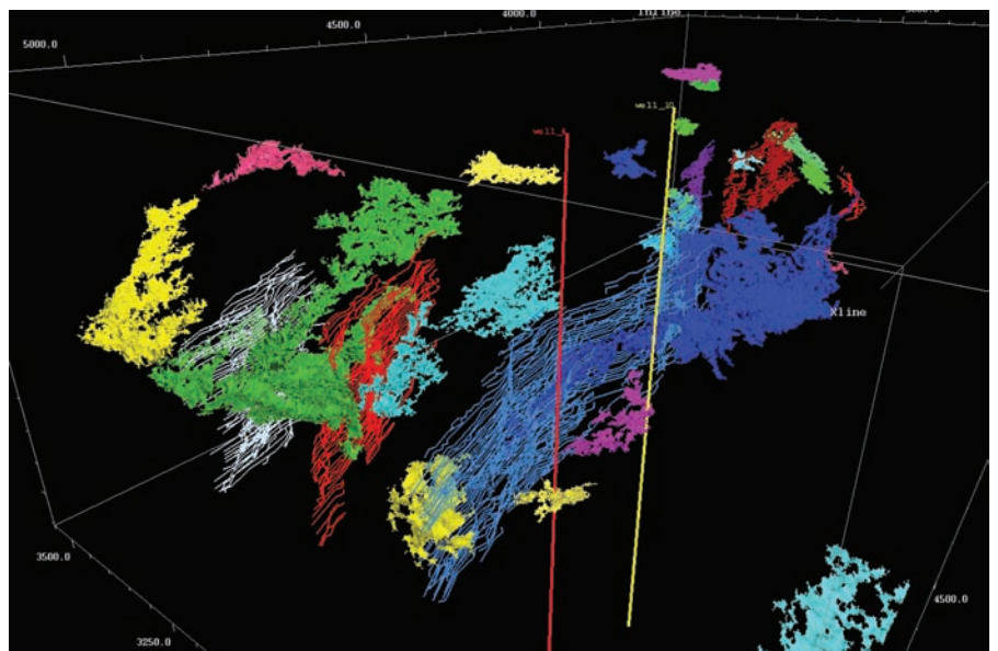
Fig 2b. The mapped geobodies (right) represent sands co-visualised with automatically extracted faults.
