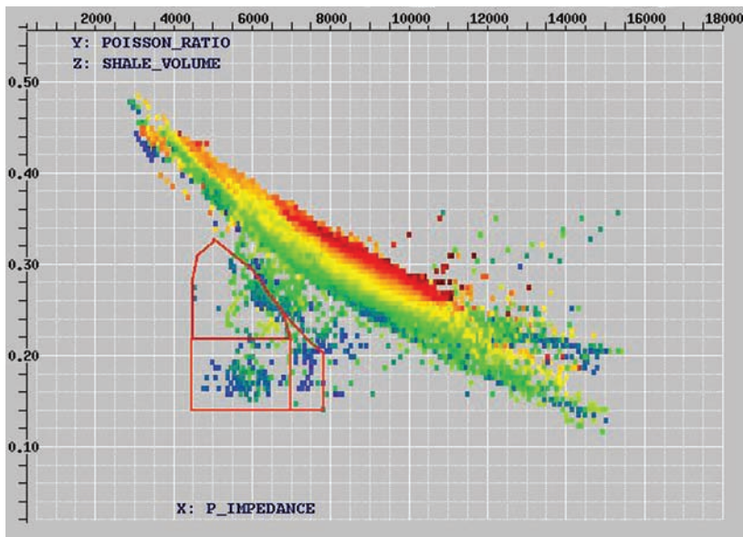
Fig 2. Crossplot of well data isolates the zone of sands using the attributes of P impedance and Poisson's Ratio. Once defined, such criteria can be applied to the seismic-generated P impedance and Poisson's ratio to predict rock property spatial distribution
