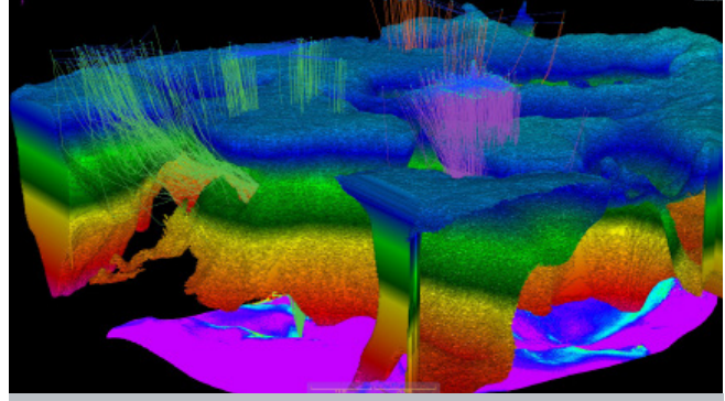
▲ Understanding subsalt uncertainty through illumination study
