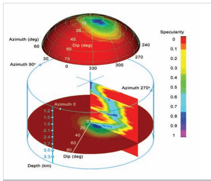
▲ “Specularity” cylindrical directional angle gather
