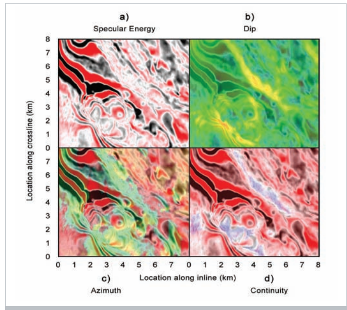
▲ Depth slice throughout 3D image: Specular weighted energy stack, and with an overlay of dip, azimuth, and continuity.
