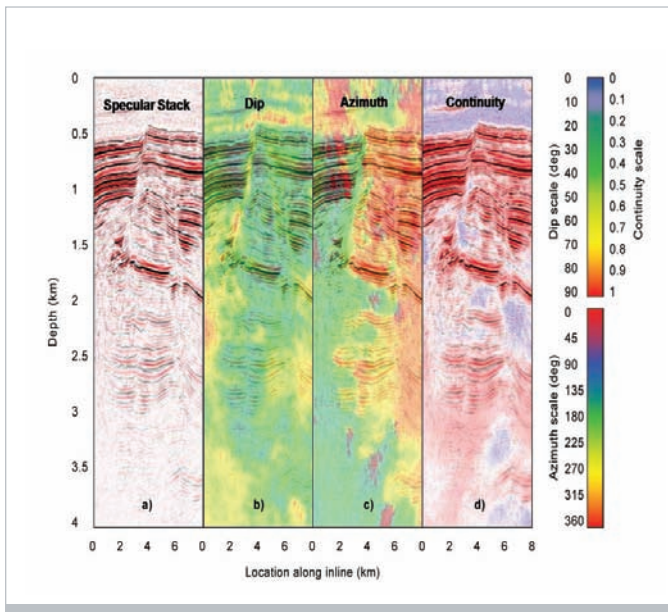
▲ Specular weighted energy stack at a given line, and with an overlay of dip, azimuth, and continuity.
