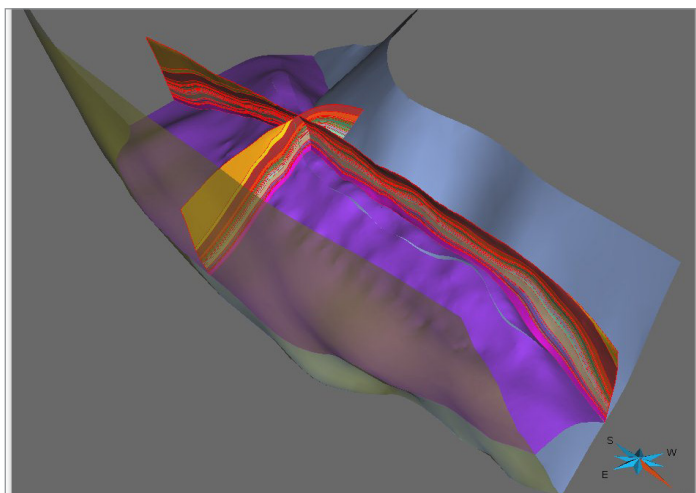
▲ Visualization of the geological grid between the main faults delimitating the reservoir
